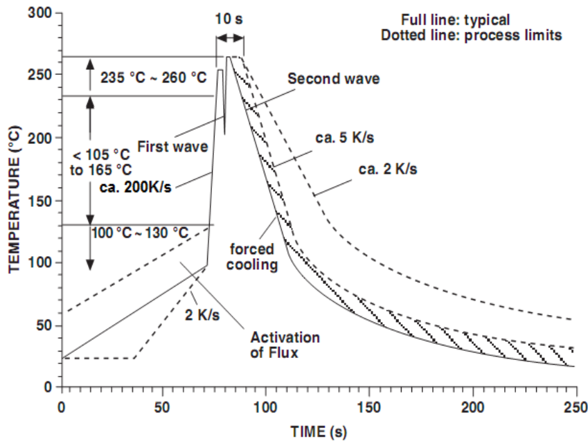
Fig. 1 - Lead (Pb)-free Wave Soldering Profile
